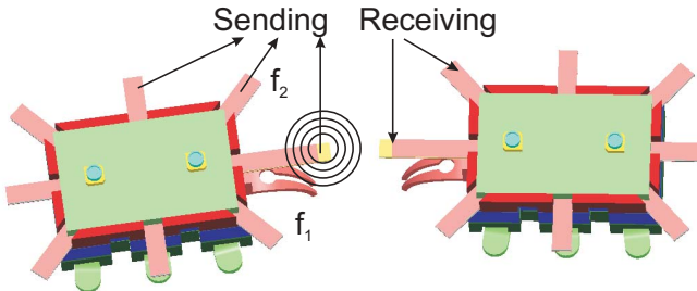
Fig. 3. Communication with a tactile sensor system.
